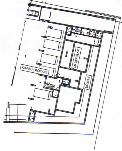
2. BODRUM KAT
